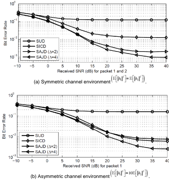
Fig. 1. BER performance of the SAJD technique the conventional techniques for varying received SNR.
