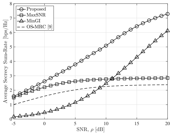
Fig. 3: Average achievable secrecy sum-rate for varying SNR when M = 2 , N = 100 , and K = 2 .
