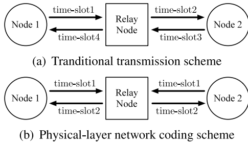
Fig. 1. Transmission schemes in two-way relaying channel.
